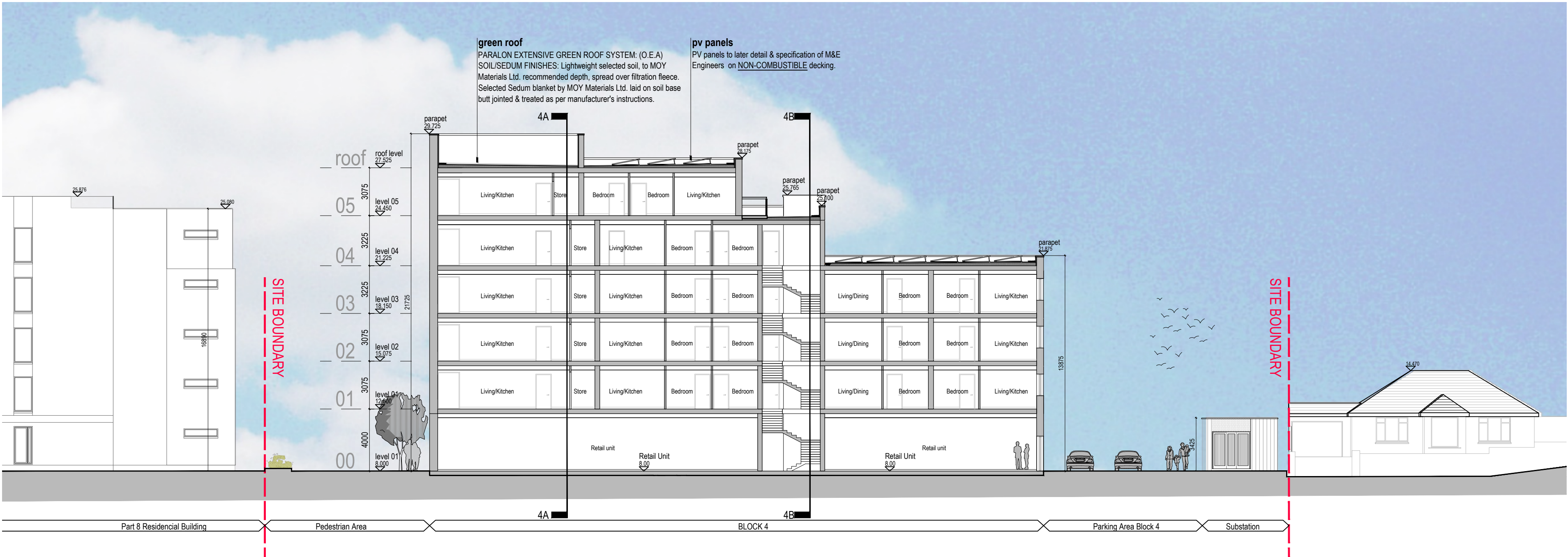
04 Block 4 SECTION 4-D 1:200
