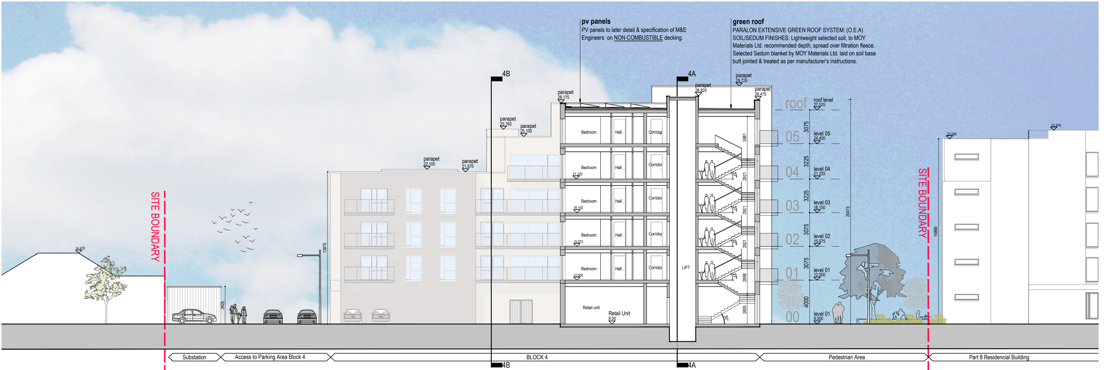
03 Block 4 SECTION 4-C 1:200
