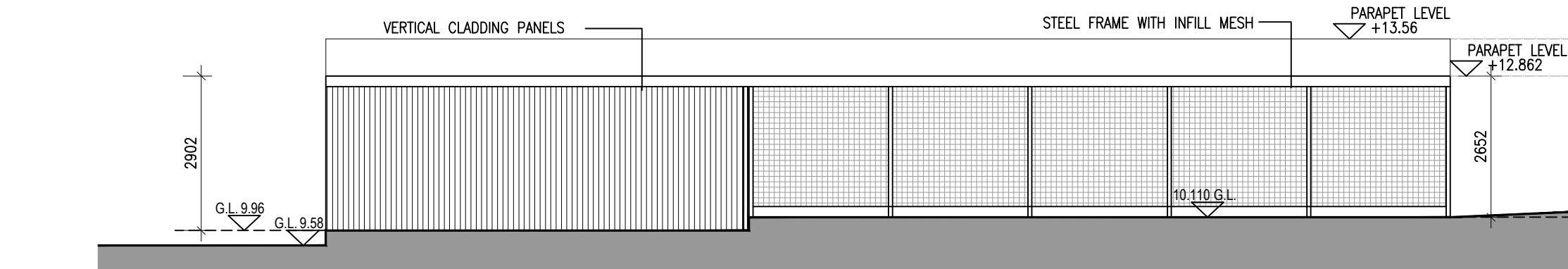
12 BIN STORE & BIKE STATION NORTH EAST FACING ELEVATION 1:100
