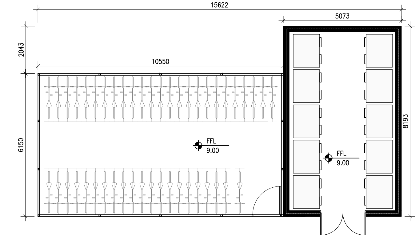
3 BIKE STATION & BIN STORE FLOOR PLAN 1:100
