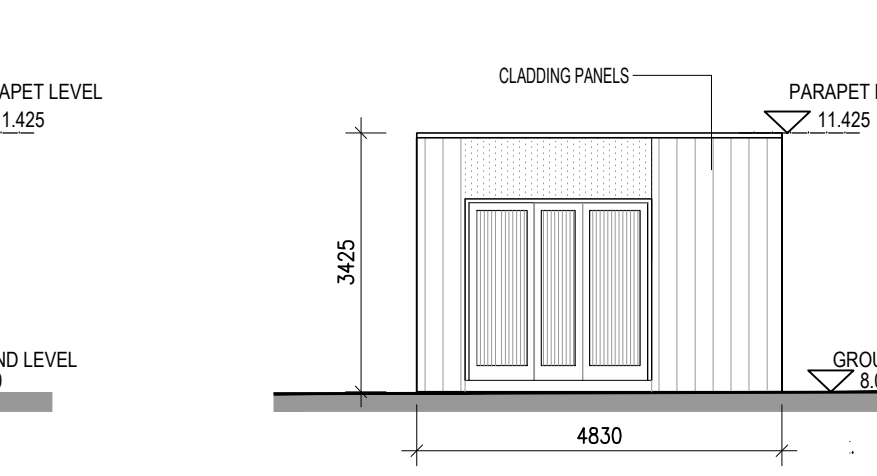
10 ESB SUBSTATION WEST ELEVATION 1:100
