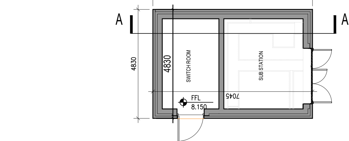
5 ESB SUBSTATION FLOOR PLAN 1:100
