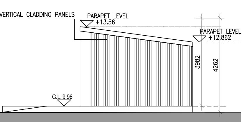
15 BIN STORE WEST ELEVATION 1:100
