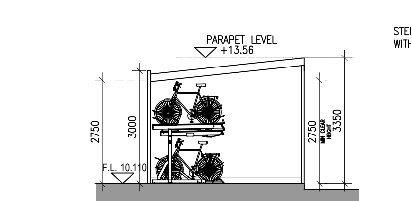
16 BIKE STATION EAST ELEVATION 1:100
