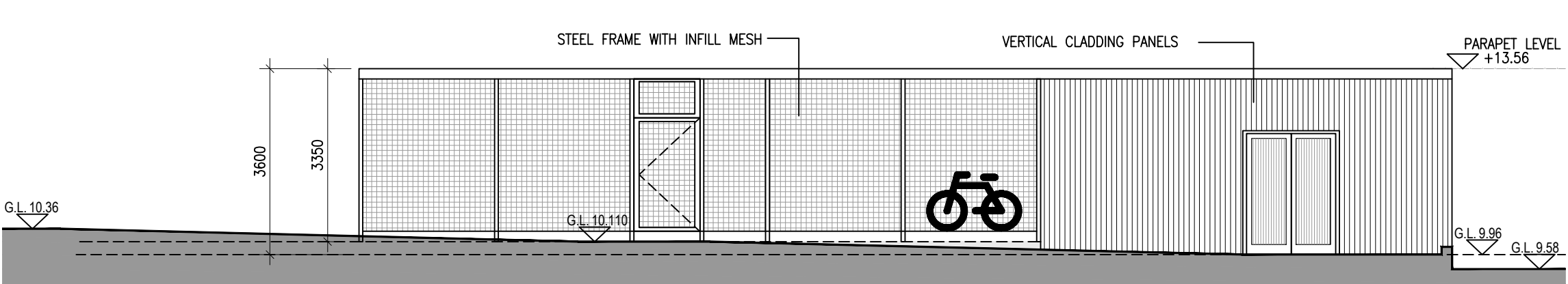
11 BIN STORE & BIKE STATION SOUTH WEST FACING ELEVATION 1:100
