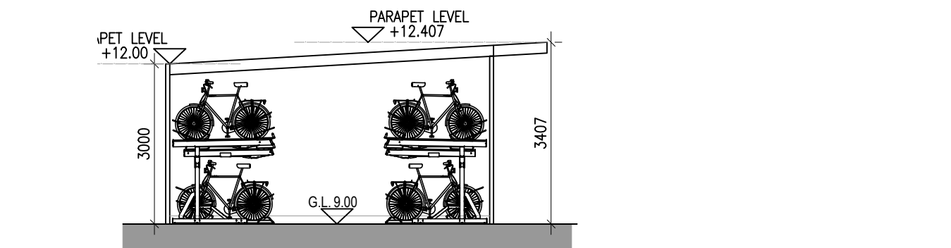
1 BIKE STATION AND BIN STORE NORTH SECTION 1:100
