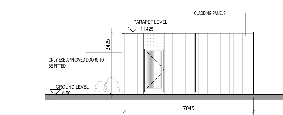
8 ESB SUBSTATION NORTH ELEVATION 1:100
