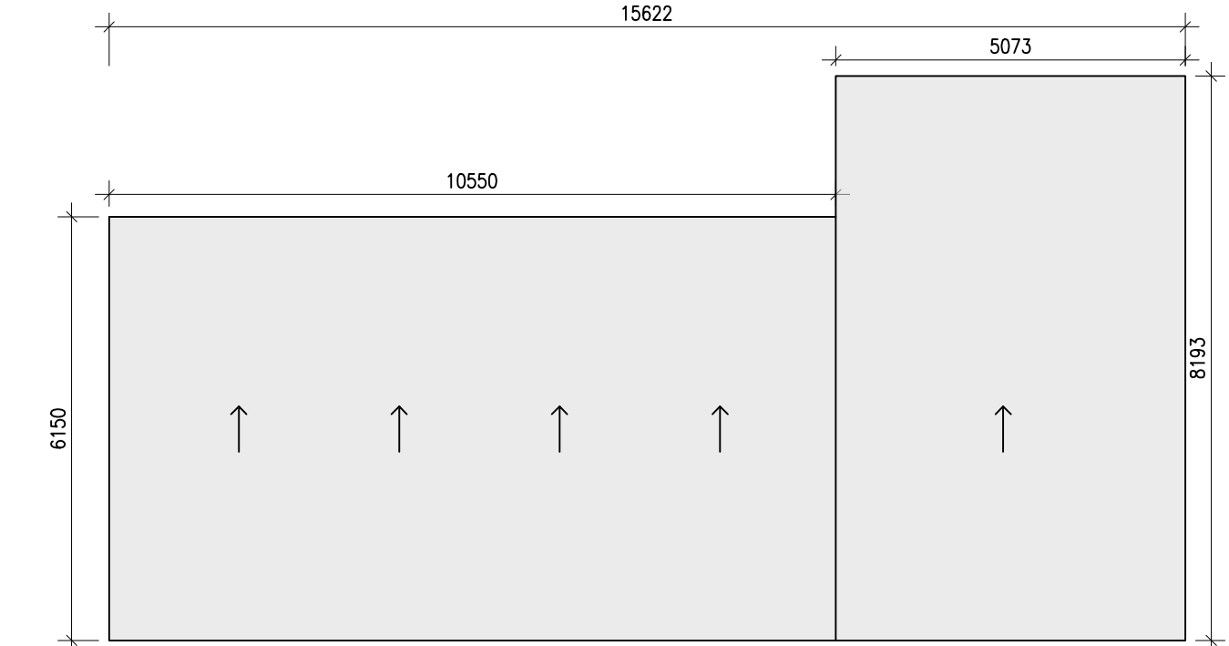
5 BIKE STATION & BIN STORE FLOOR PLAN 1:100
