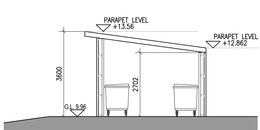
14 BIN STORE WEST SECTION 1:100
